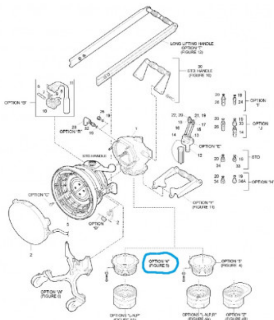
Figure 1 64910 Hydrant Coupler & Options
